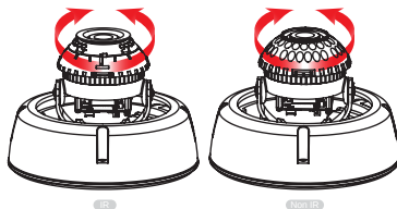
2 Panning 360°
